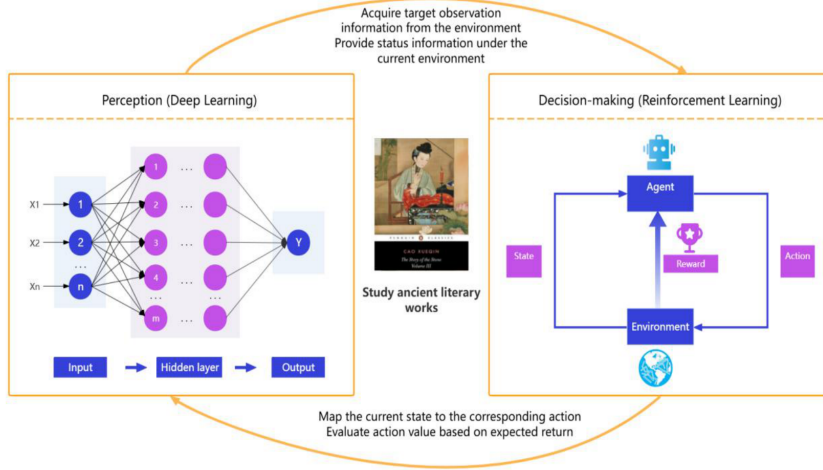
FIGURE 2. Reinforcement learning framework
