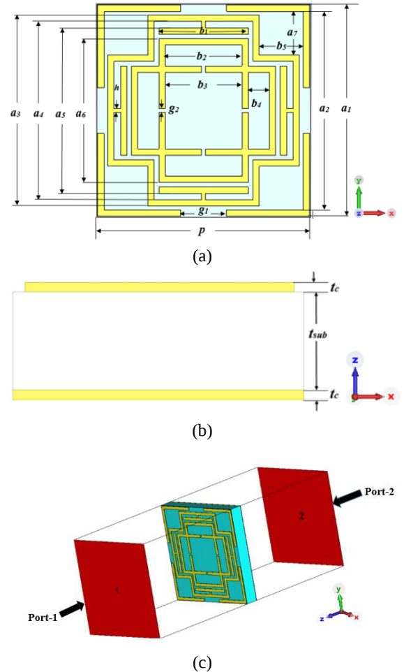
FIGURE 1. (a) Top, (b) Side, and (c) Perspective views of the proposed microwave metamaterial absorber.
