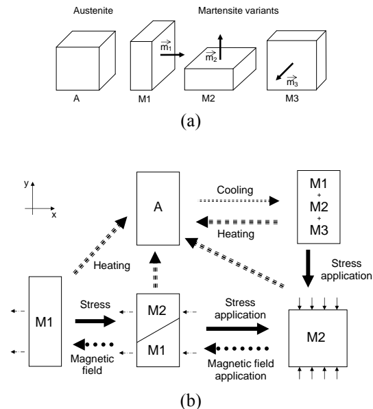
Figure 1: MSMA behaviour: (a) austenite phase and the three martensite variants and (b) martensitic reorientation: effects of mechanical stress, magnetic field and temperature.
